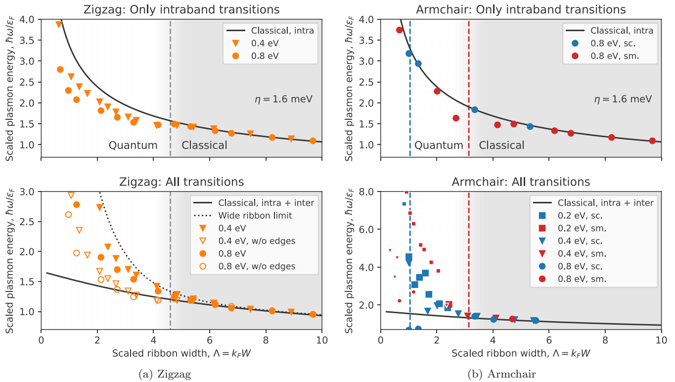
FIG. 4. Scaled plasmon energy as a function scaled ribbon width \Lambda . The value \Lambda = 5 corresponds for example to a width of 16.4 nm for \epsilon_F = 0.2 eV. (a) \Lambda is varied by changing W while keeping the Fermi energy fixed at either 0.4 eV (triangles) or 0.8 eV (dots). The vertical dashed line corresponds to \Lambda_c^z \simeq 4.6 . The open symbols in the bottom panel correspond to calculations of plasmon energies where edge states were removed from the calculation. (b) Top: The intraband plasmons of AC ribbons, both the classical prediction and the quantum plasmon predictions for semiconducting and for semimetal ribbons. Blue and red dashed vertical lines correspond to \Lambda_c^{ac} = \pi/3 and \pi , respectively. (b) Bottom: As in the top panel, but now including all transitions. The small symbols are used for the peaks in the loss spectrum that are not associated with an actual plasmon defined as \text{Re}(\epsilon_n) = 0 .
