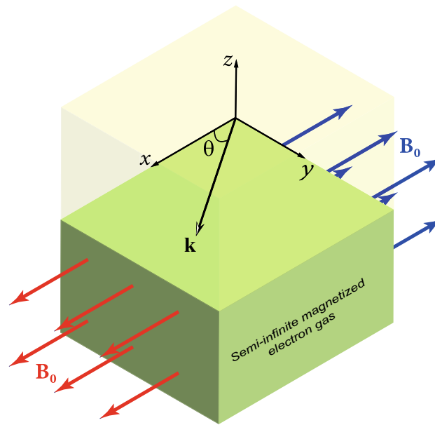
Figure 1. Sketch of a semi-infinite magnetized electron gas with static magnetic field \mathbf{B}_0 parallel to the surface. Here we choose the direction of \mathbf{B}_0 fixed along the +\mathbf{e}_x (red vectors) or -\mathbf{e}_x (blue vectors). Note that \mathbf{e}_x is the unit vector along the x -axis. Also, \mathbf{k} is the wavevector of the propagating surface wave, and \theta (or 180^\circ - \theta ) is the angle between \mathbf{k} and \mathbf{B}_0 . The special cases \theta = 0 (or 180^\circ ) and \theta = 90^\circ are called the Faraday and Voigt configurations, respectively. Here we study magnetoplasmons for the general case of arbitrary \theta , which we call a mixed Faraday–Voigt configuration. Note that in the Voigt configuration the magnetoplasmons travel in the +\mathbf{e}_y direction. The electron gas is bounded from above by a semi-infinite insulator at z = 0 .
