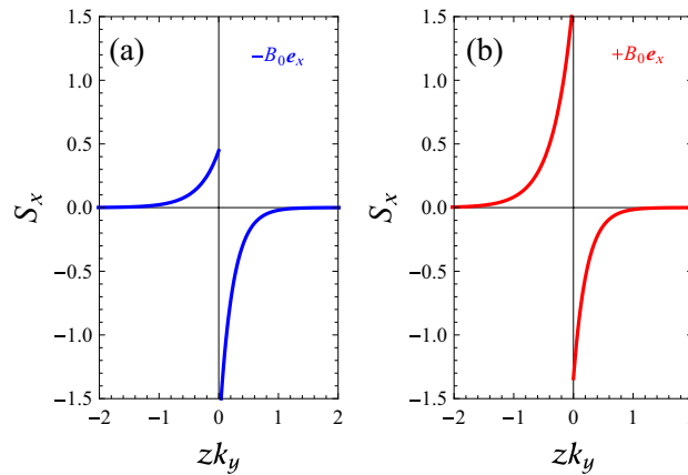
Figure 7. Normalized profile S_x(z) of SMP modes of a flat magnetized electron gas-vacuum interface, as obtained from Eq. (16) when k_x/k_y = 2 , k_x > 0 , and k_y is a positive constant, corresponding to the labeled points in Fig. 3a. (a) \mathbf{B}_0 = -B_0 \mathbf{e}_x . (b) \mathbf{B}_0 = +B_0 \mathbf{e}_x .
