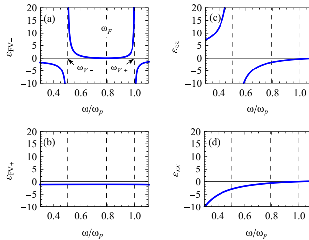
Figure 2. Variation of (a) \varepsilon_{FV-} , (b) \varepsilon_{FV+} , (c) \varepsilon_{zz} , and (d) \varepsilon_{xx} , with respect to the dimensionless frequency \omega/\omega_p , when \varepsilon_1 = 1 , and \omega_c = 0.5\omega_p .
