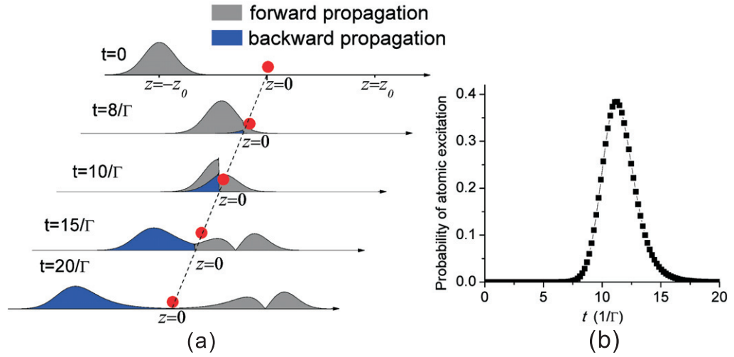
Figure 2. (a) Snapshots of the amplitudes of the transmitted and reflected wavepackets as distributed along the spatial axis at different instances of time; (b) the time dependence of the atomic excitation. At t = 0 , the peak of the Gaussian input single-photon wavepacket is localized at z = -Z_0 = -10v_g/\Gamma , with FWHM equal to \Gamma . The red dot indicates the fixed position of the emitter.
